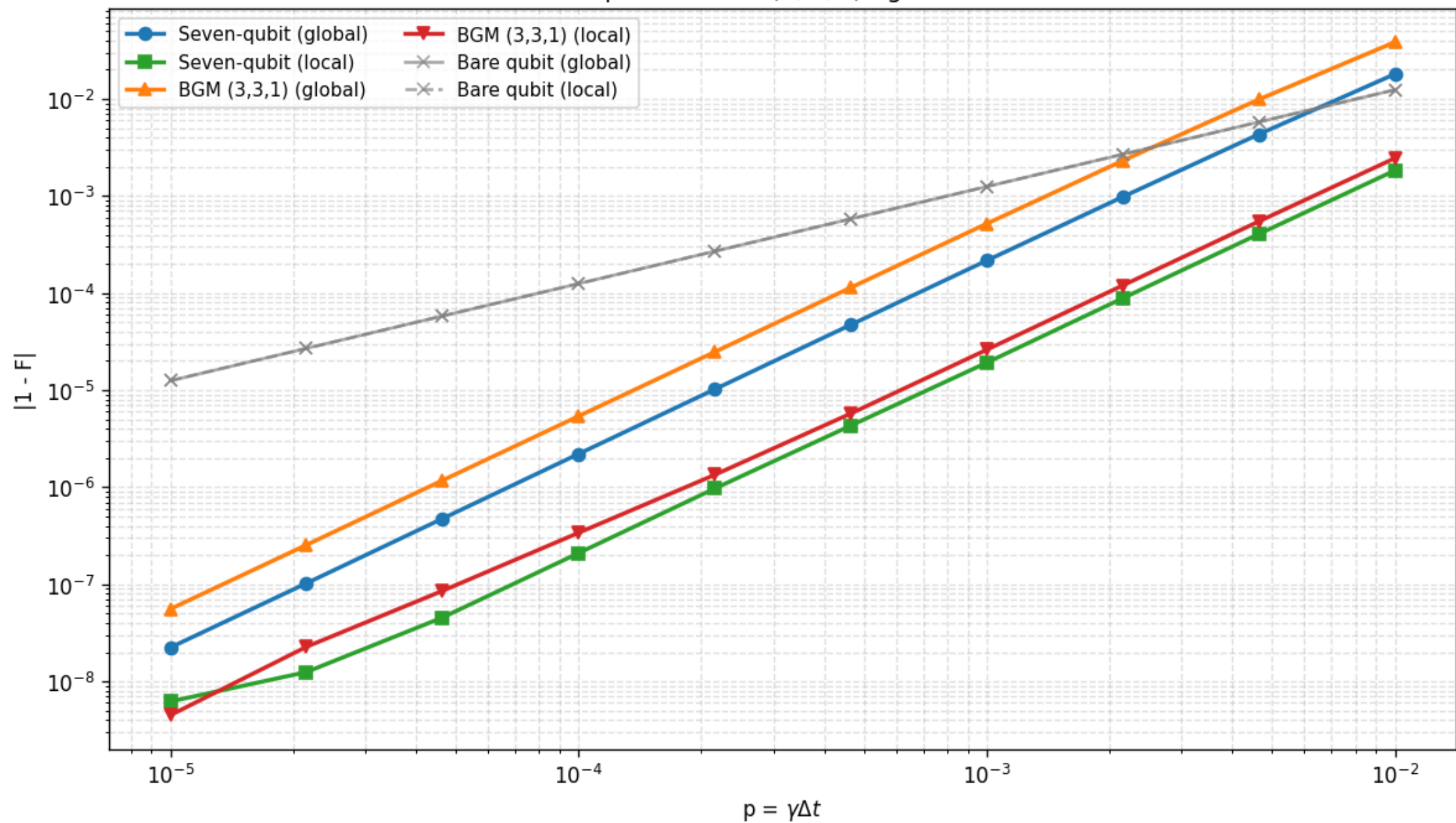
7-qubit code vs (3, 3, 1) bgm code
